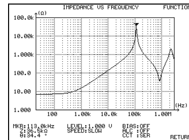
Impedance plotted against frequency
